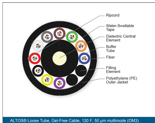
ALTOS® Loose Tube, Gel-Free Cable, 120 F, 50 µm multimode (OM3)
