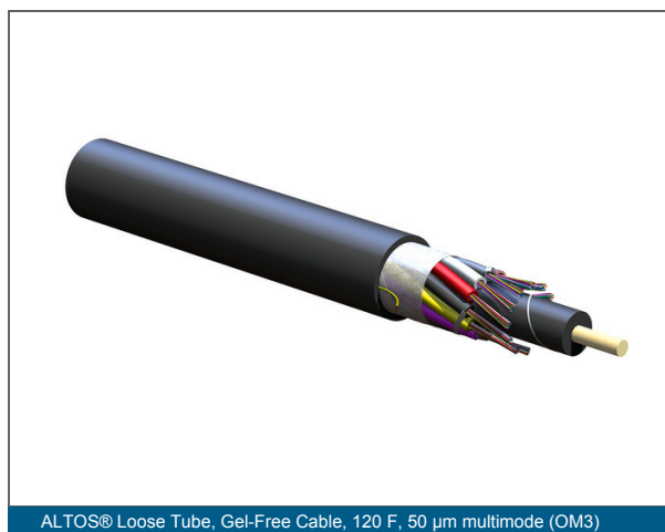
ALTOS® Loose Tube, Gel-Free Cable, 120 F, 50 µm multimode (OM3)
